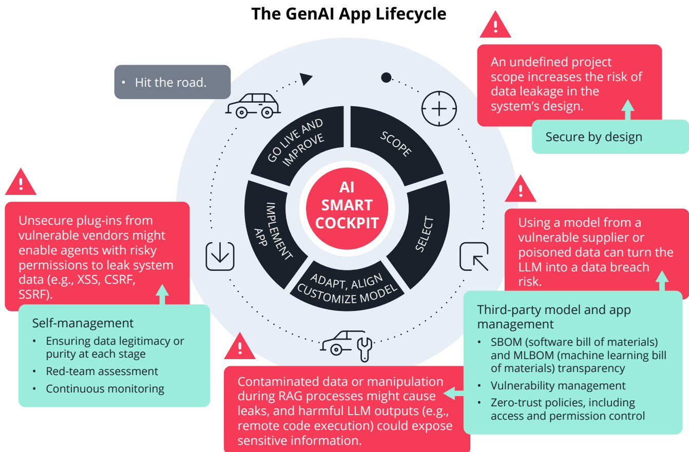
Figure 4. Secure-by-design principles, transparent third-party model management, and robust self-management practices help mitigate risks in the GenAI app lifecycle.
