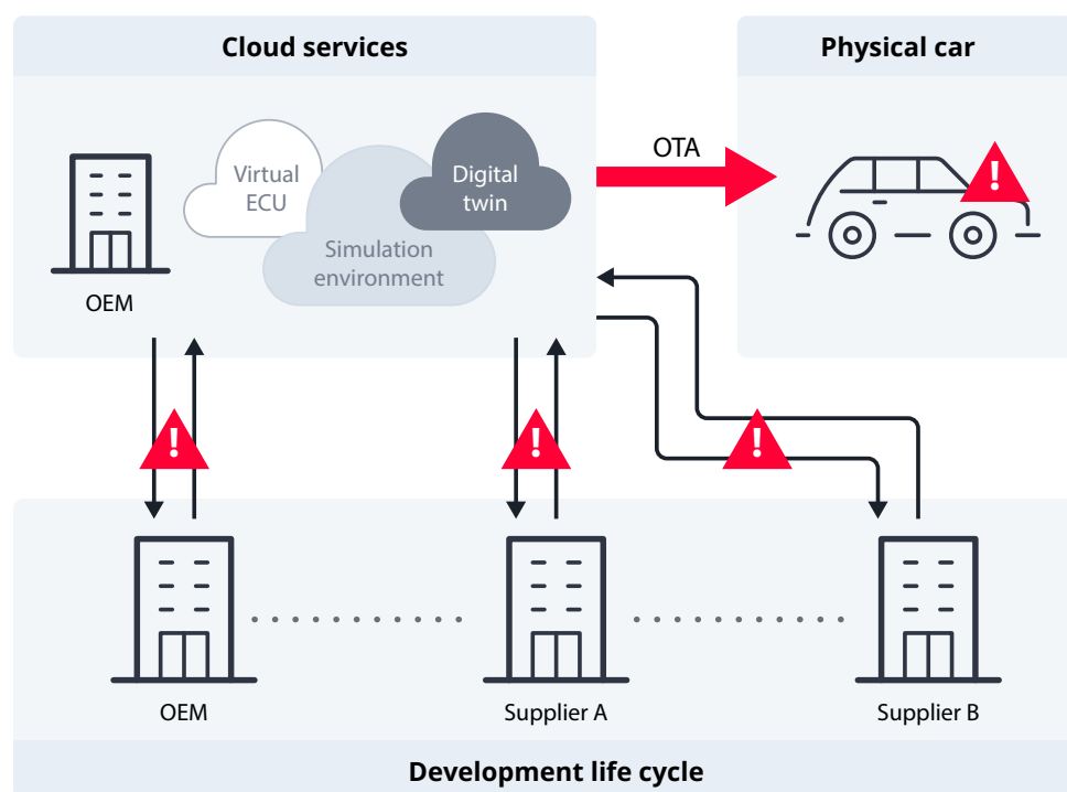
Figure 4. Risks in the SDV ecosystem
