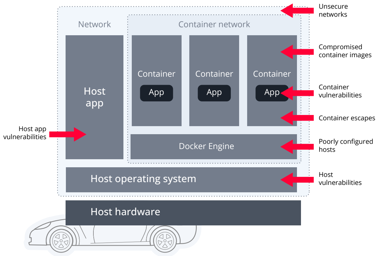
Figure 3. Container attack vectors
